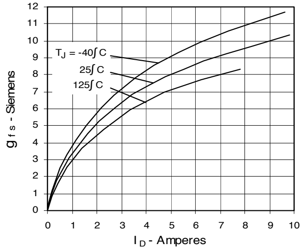
Fig. 8. Transconductance
